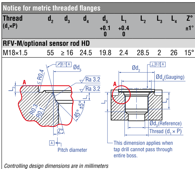
Fig. 34: Notice for metric threaded flange M18×1.5-6g based on DIN ISO 6149-1
