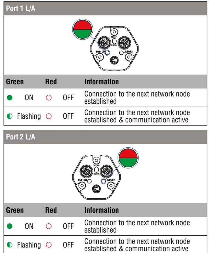
Fig. 82: LED status display, part 3
