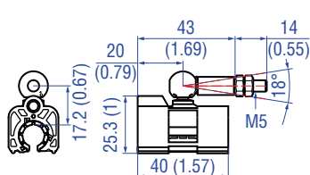
Magnet slider S, joint at top Part no. 252 182
