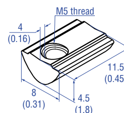
T-nut Part no. 401 602
