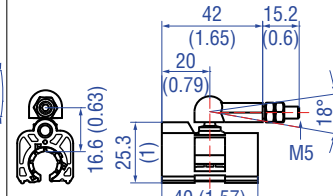
Magnet slider G, backlash free Part no. 253 421
