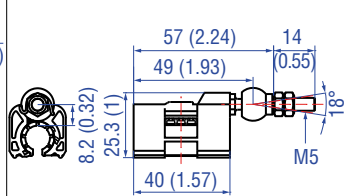
Magnet slider V, joint at front Part no. 252 184
