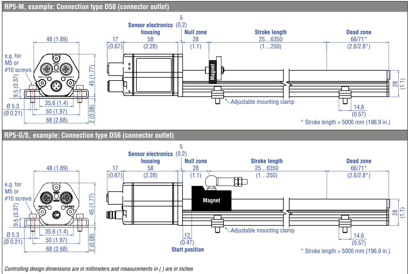
Fig. 3: Temposonics® RP5 with U-magnet and magnet slider
