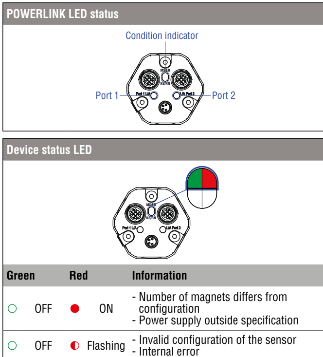
Fig. 80: LED status display, part 1
