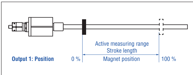
Fig. 31: Active measuring range
