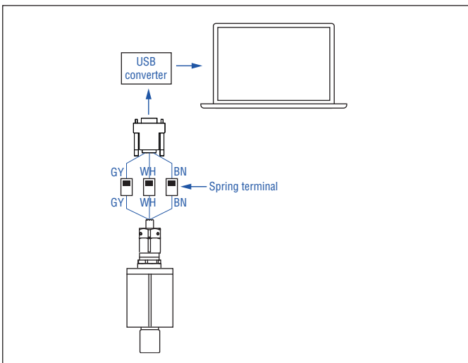
Fig. 32: Connect PC programmer
