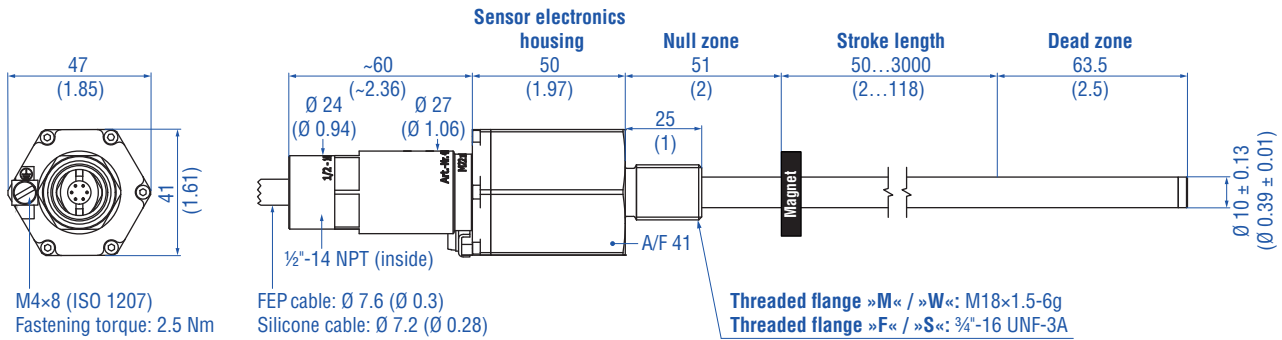
Fig. 4: Temposonics® ET (rod sensor) with ring magnet
