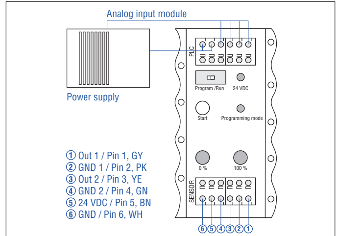
Fig. 29: Connect cabinet programmer (see connector wiring Fig. 21)
