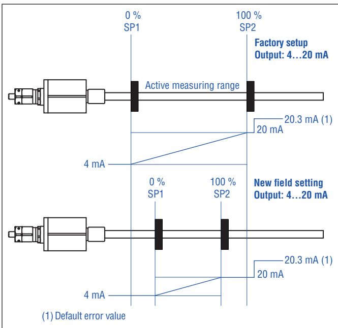
Fig. 37: Adjust start and end position
