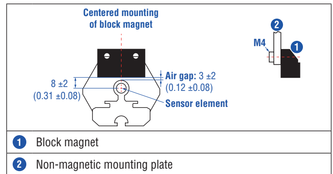
Fig. 14: Mounting of block magnet (part no. 403 448)
