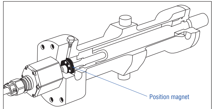
Fig. 6: Sensor in cylinder
