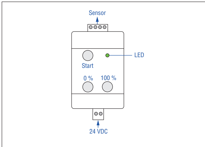
Fig. 25: Adjust measuring range
