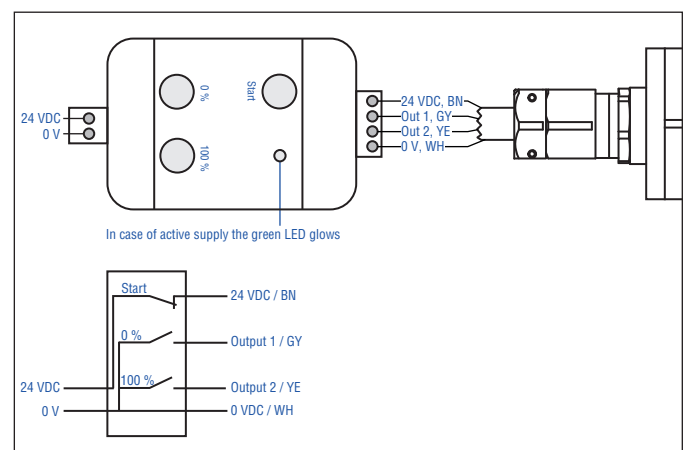
Fig. 24: Connect hand programmer (see connection wiring Fig. 21)
