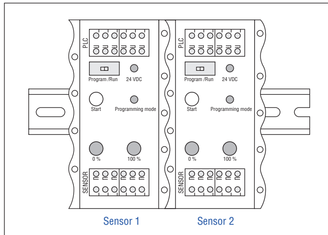
Fig. 28: Dimensions: 10 × 55 × 31 mm (0.39 × 2.17 × 1.22 in.); material: Aluminum, side caps PA 6.6 FR; connection type: Spring terminals, max. 1.5 mm 2 ; ingress protection: IP20
