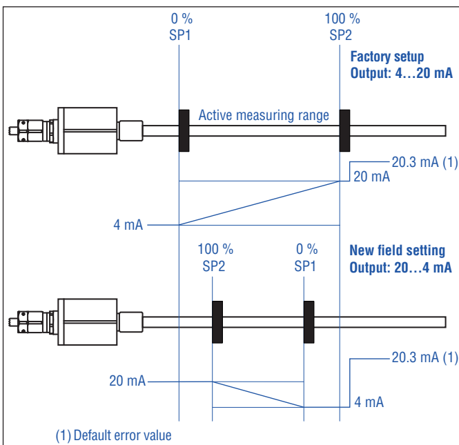
Fig. 38: Start and end position, adjustment/reversal of measuring direction
